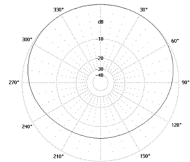
Radiation pattern – H plane
